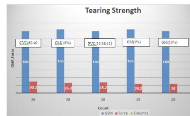
Figure : Graphical representation of tearing strength
